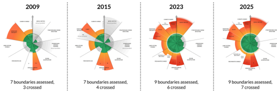
(Credit: Azote for Stockholm Resilience Centre, Stockholm University. Based on Sakschewski and Coesar et al. 2025, Richardson et al. 2023, Steffen et al. 2015, and Rockström et al. 2009).
